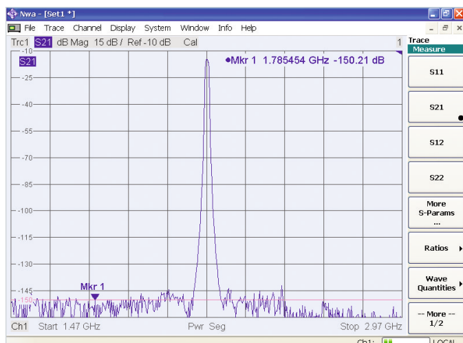
Typical dynamic range with direct receiver access.
